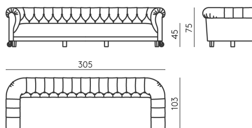
DIVANO L CM 305 _ CON RUOTE ANTERIORI SOFA L CM 305 _ WITH FRONT CASTORS
