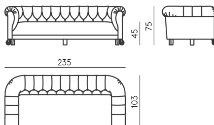
DIVANO L CM 235 _ CON RUOTE ANTERIORI SOFA L CM 235 _ WITH FRONT CASTORS
